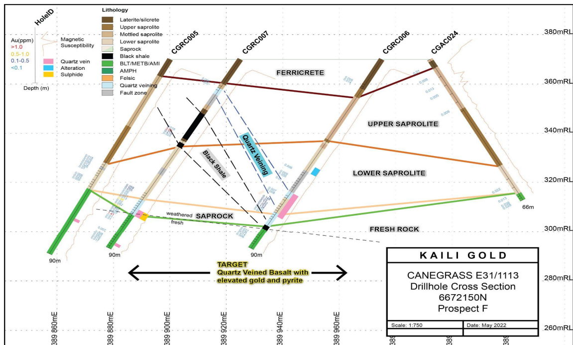
Figure 10: RC Interpreted Drill Cross Section 6672150N.
