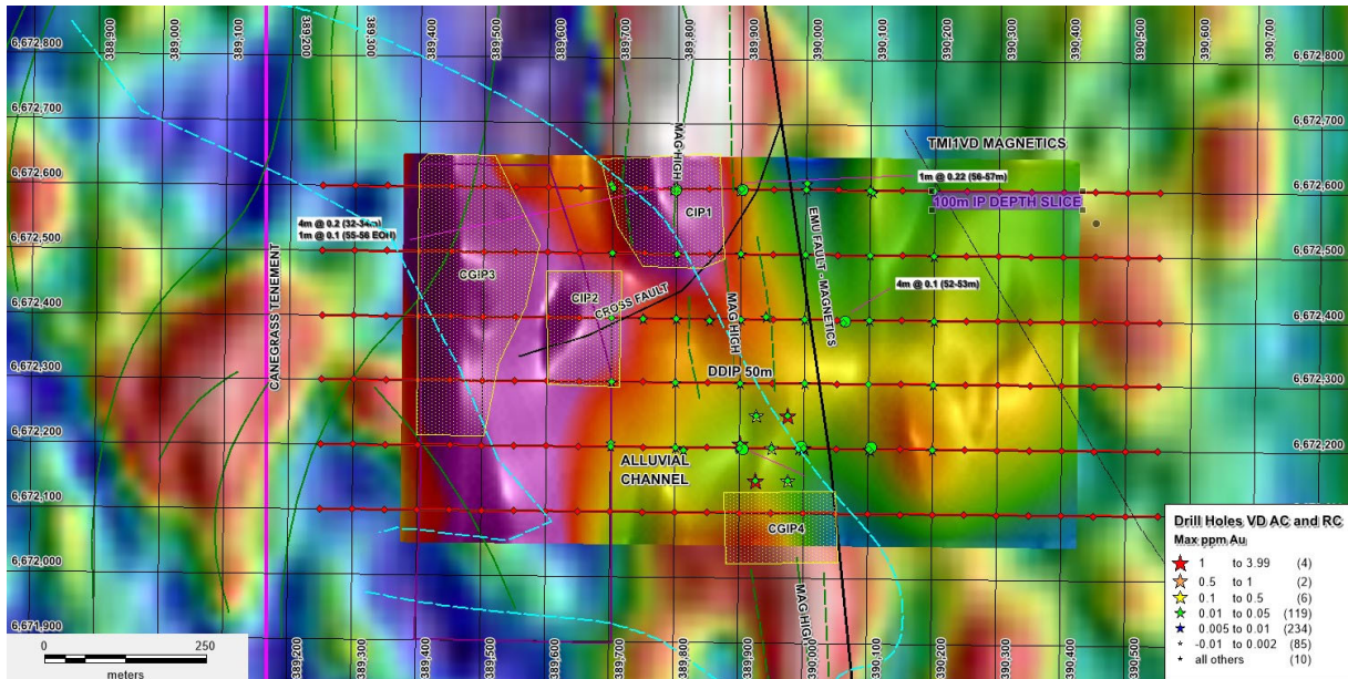
Figure 6: Canegrass Prospect F showing the 4 IP Conductive Target Areas CGIP 1 to 4 with the IP Survey overlaid on the TMI Aeromagnetics – Depth Slice -100 m
