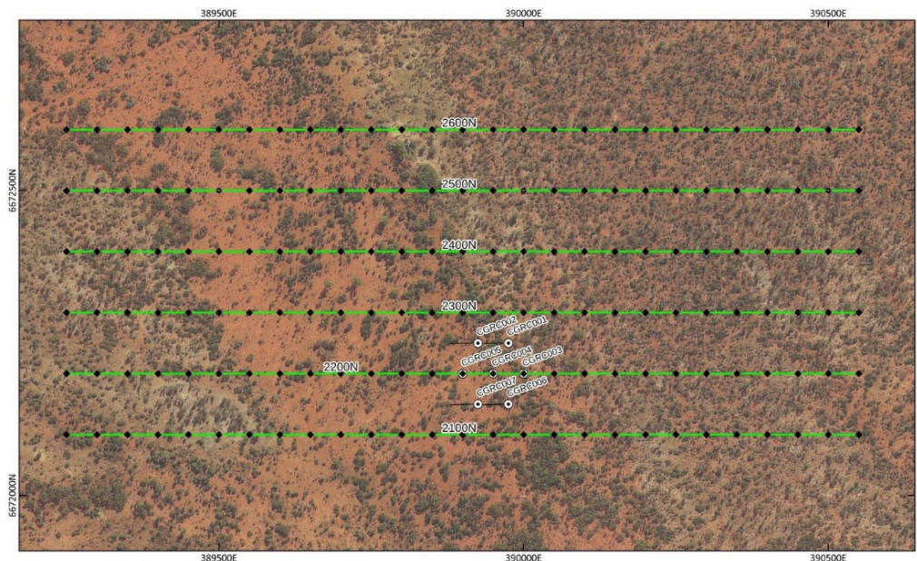
Figure 7: Canegrass Prospect F DDIP 2022 Survey Location Map (GDA94/MGA51). Black dots are DDIP electrode locations. Existing drill collars and traces shown for reference.
