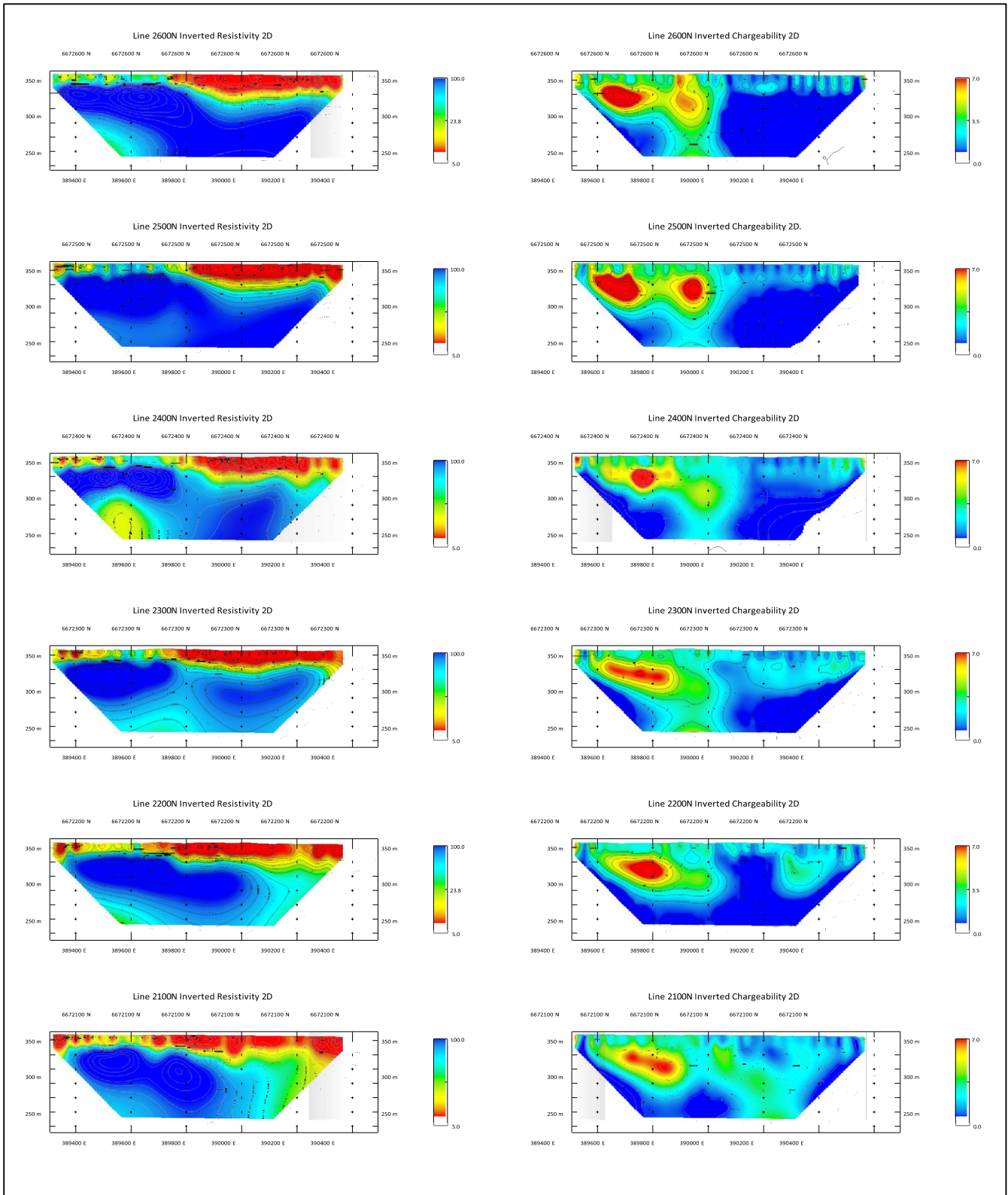
Figure 9. Canegrass DDIP Survey – 2D Model Sections for all lines.
