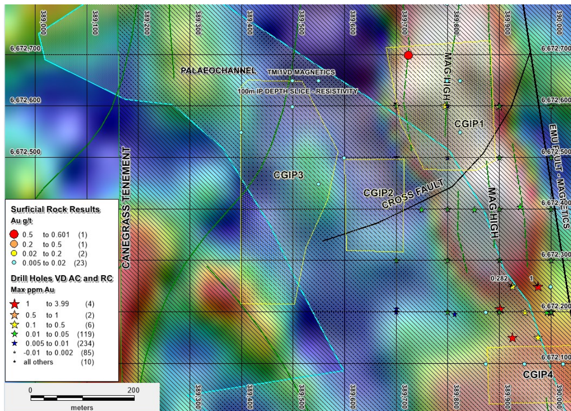
Figure 3: Targets CGIP 1 to 4 with surface rock sample sites on TMI 1VD Magnetics
