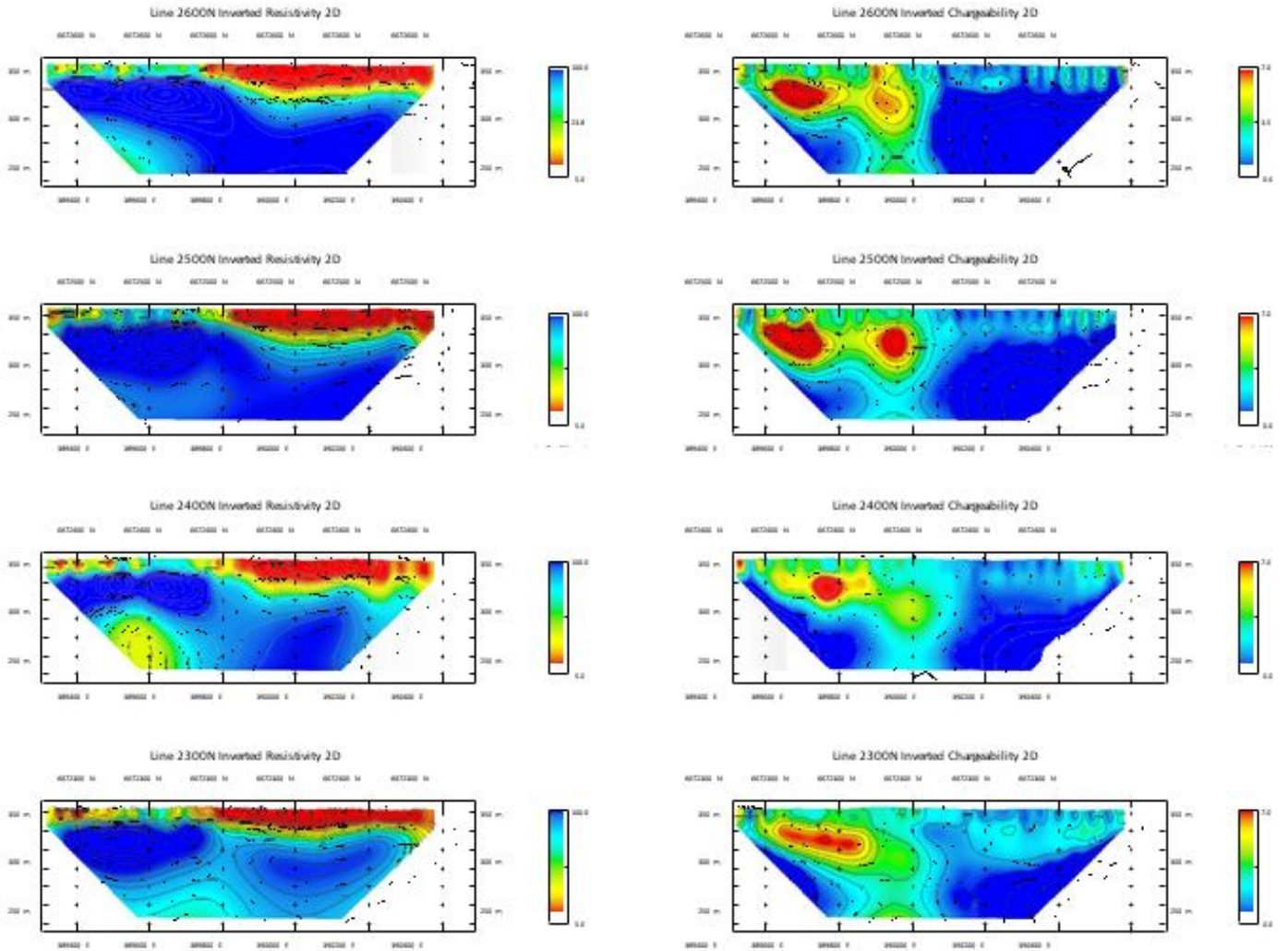
Figure 5: IP Cross Sections 6672600N to 6672300N – Resistivity left and Chargeability right.
